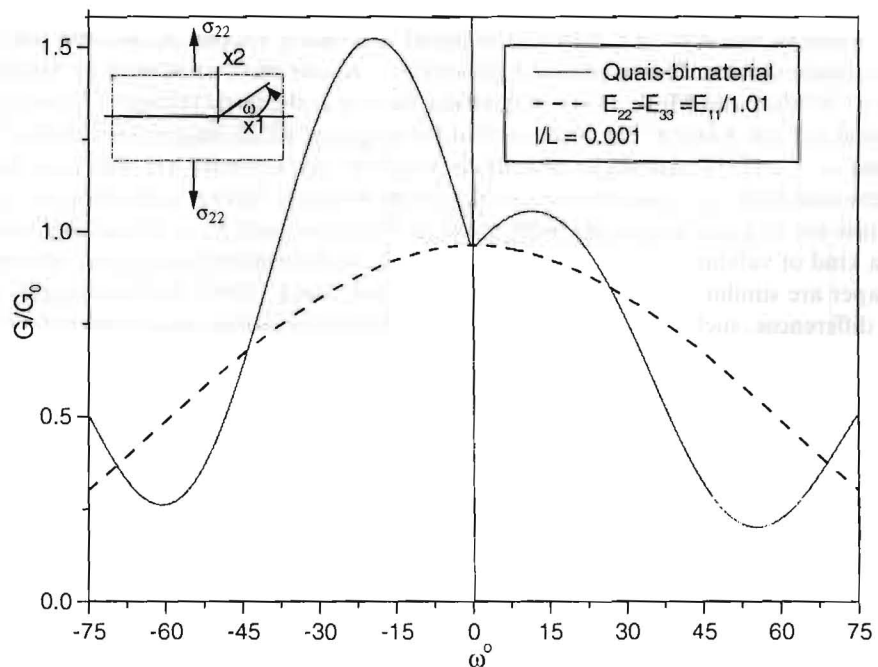
Fig. 9. Energy release rate for the branched crack vs. branching angle for a quasi-bi-material under pure tension loading.
