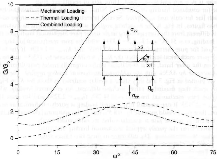
Fig. 7. Energy release rate for an anisotropic bi-medium ( \theta_1 = 30^\circ , \theta_{11} = -120^\circ ).
