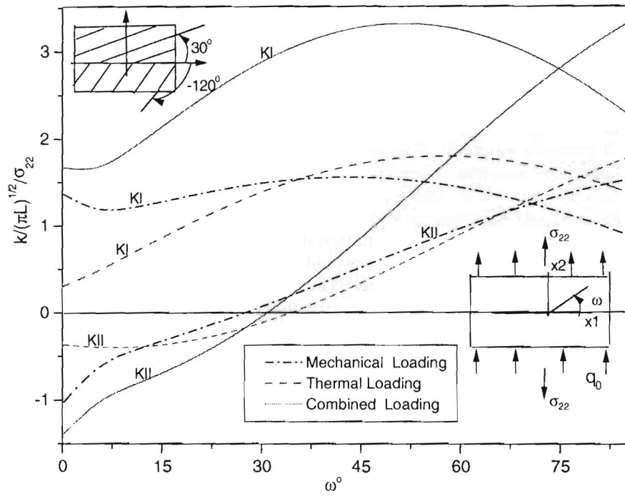
Fig. 6. Stress intensity factors for an anisotropic bi-medium ( \theta_1 = 30^\circ , \theta_{11} = -120^\circ ).
